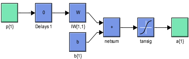
Figure 7. Architecture of layer 1.
