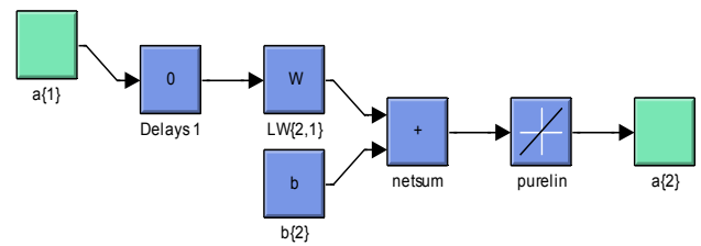
Figure 8. Architecture of layer 2.
